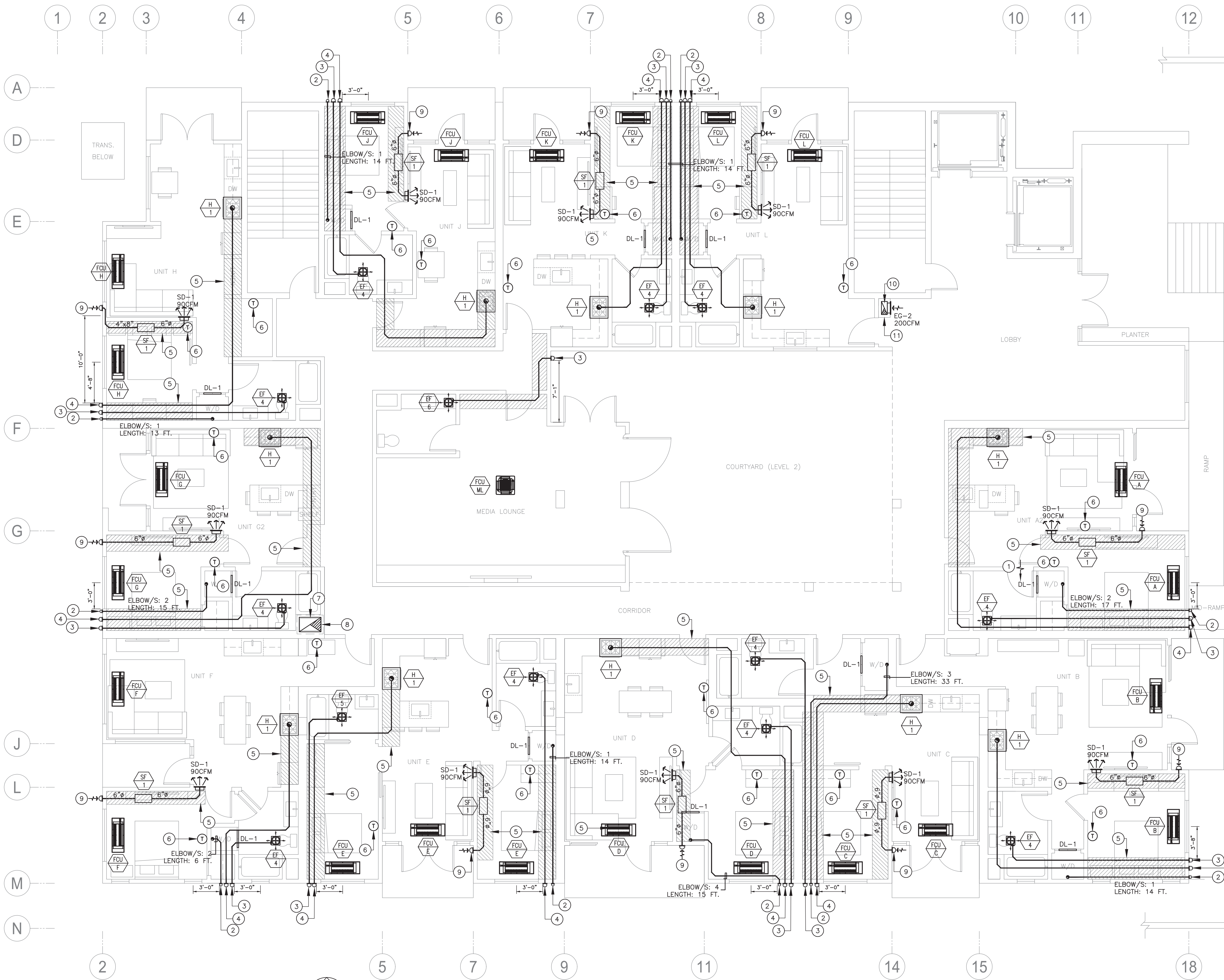
MECHANICAL LEVEL 1 PLAN SCALE: 3/16"=1'-0"
