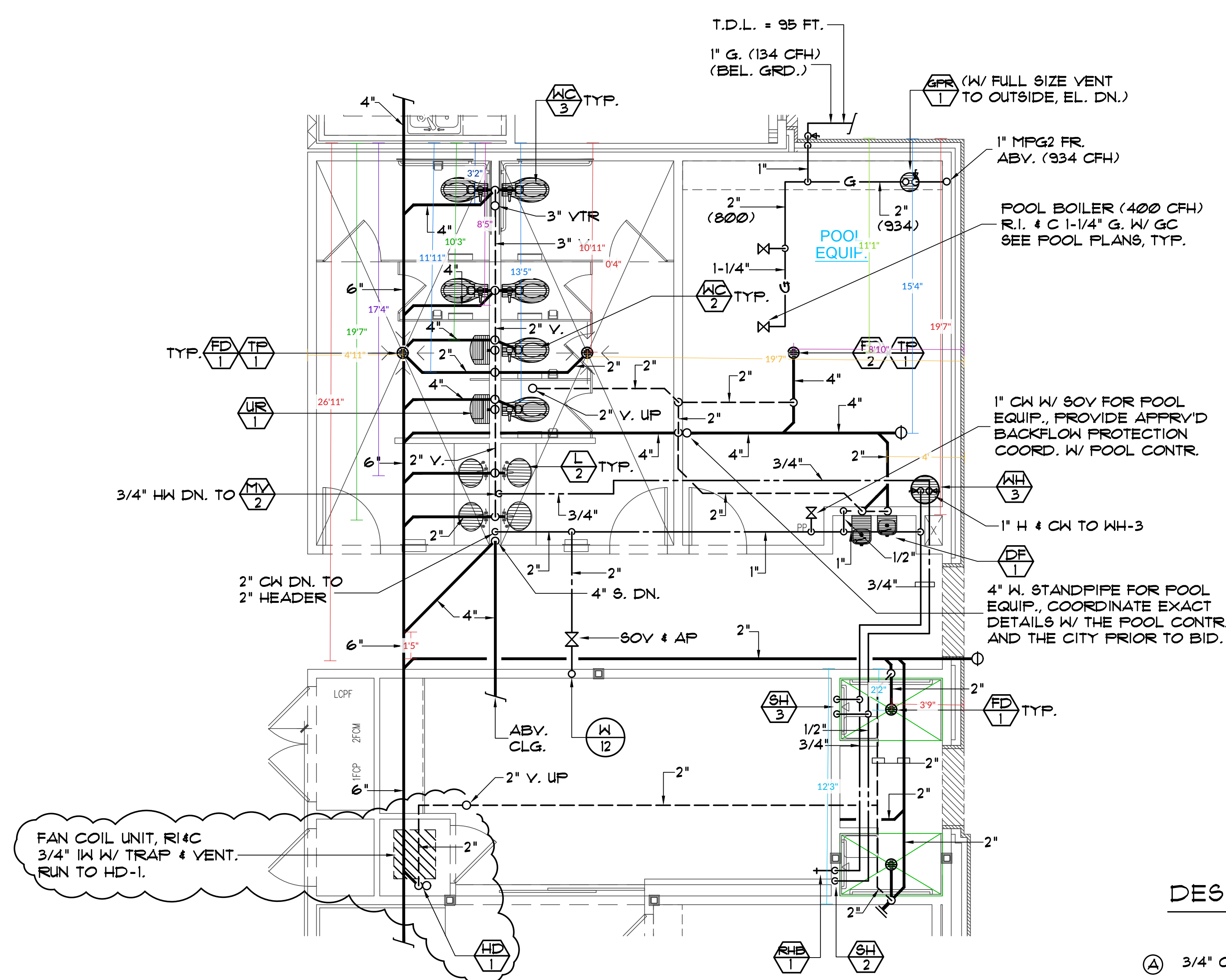
PLUMBING ENLARGED PLAN SCALE: 1/4" = 1'-0"
