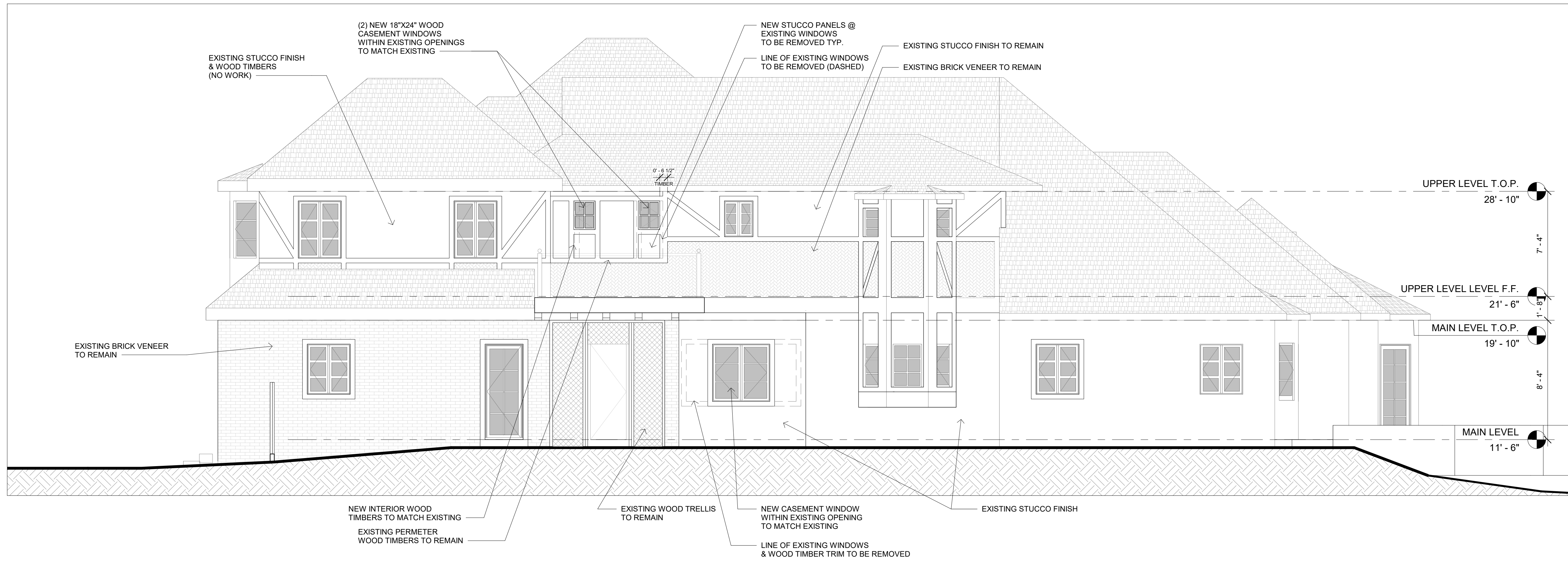
1 SOUTH ELEVATION 1/4" = 1'-0"
